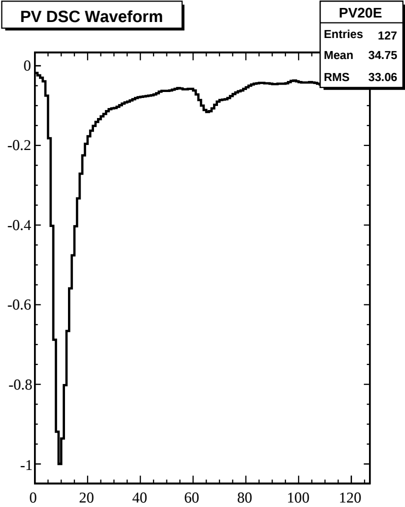
PV DSC Waveform
