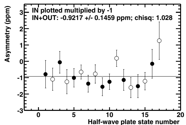
FIG. 1. Results for the detector yield asymmetry (average of ten detectors). Each data point represents the average between two half-wave plate state changes. The OUT data are plotted as filled circles and the IN data as open circles. The sign of the IN data is reversed to give the correct sign.
