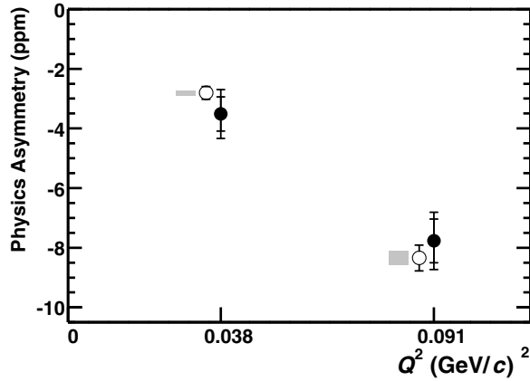
FIG. 2. The physics asymmetries measured in SAMPLE II (updated results) and SAMPLE III are plotted as a function of Q^2 (solid circles). Also plotted (with offset Q^2 for visibility) are the theoretical predictions with the value of G_A^e taken from Ref. [8], and G_M^s = 0.15 (open circles). The height of the gray rectangles represents the change in the physics asymmetry corresponding to a 0.6 change in G_M^s .
