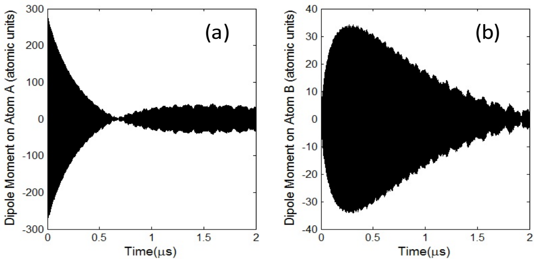
Figure 6.5: Calculated average dipole moment on individual atoms for coupled via DD interactions. The plots are analogous to those shown in Figure 6.2, but a random ensemble. The density of the ensemble is \sim 2 \times 10^9 \text{ cm}^{-3} . Compared to Figure 6.3, macroscopic coherence is quickly lost because of the dephasing of the wavepackets on different atom pairs.
