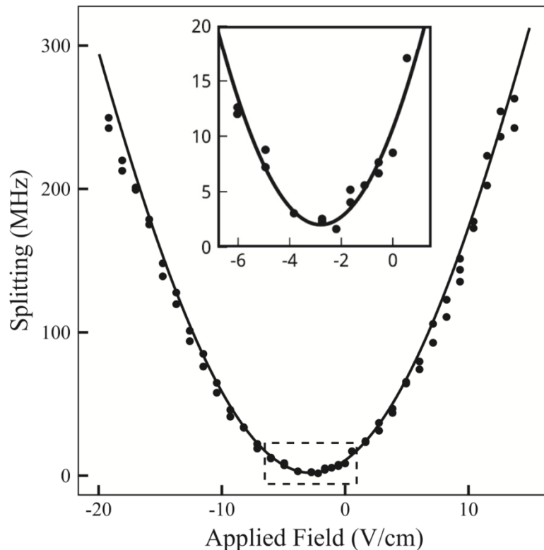
Figure 4.4: Difference (i.e., splitting) in the transition energies for exciting 32p_{3/2} |m_j|=1/2, 3/2 from 5p_{3/2} as a function of applied electric field. Filled circles are measurements and the solid curve is the result of a numerical Stark map calculation assuming orthogonal “offset” and “residual” electric field components due to the MCP of 2.8 and 1.5 V/cm, respectively. The inset shows a magnified view of the portion of the main figure within the dashed window.
