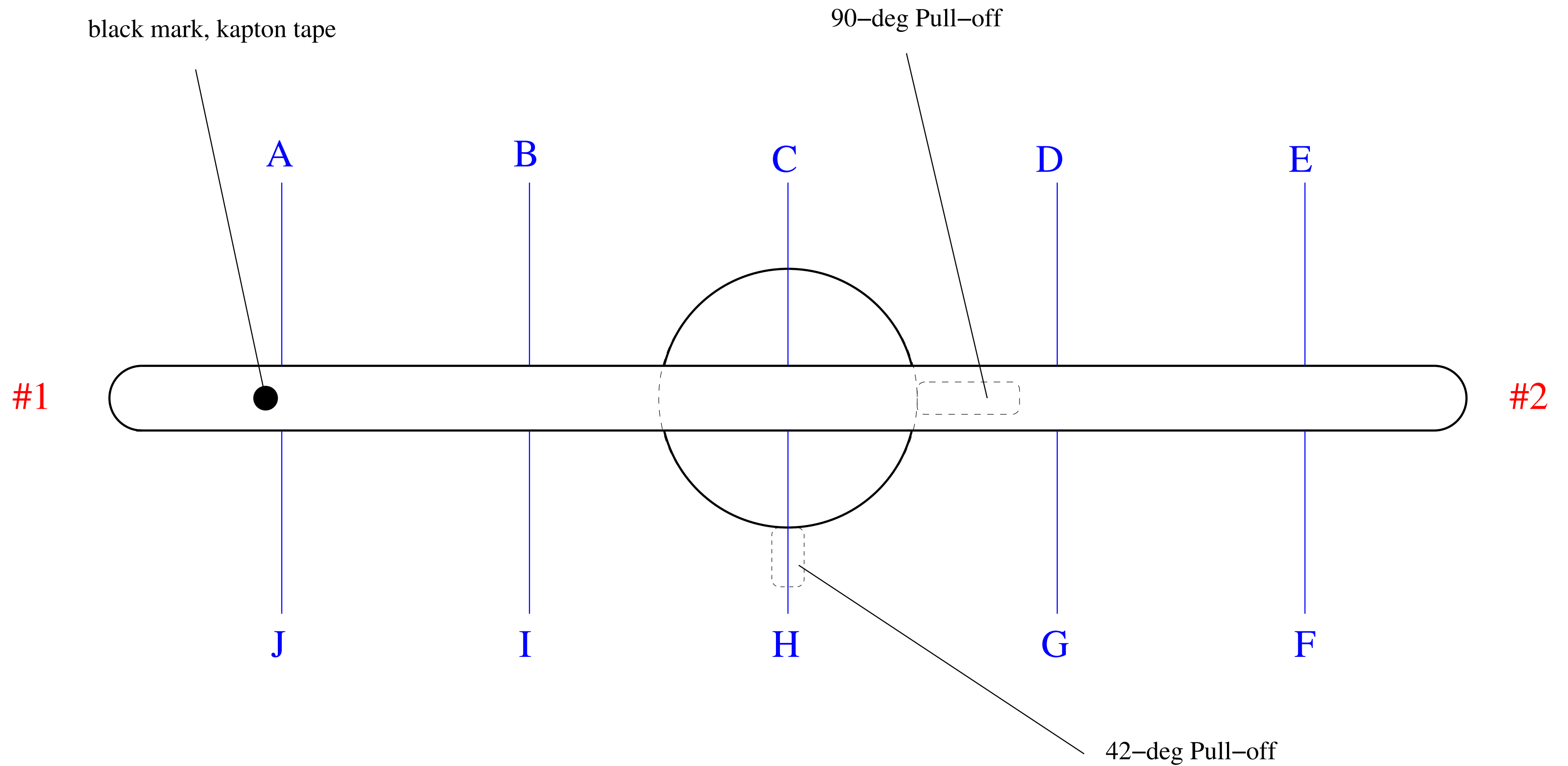
Cell Orientation looking into Bottom of Target Chamber
