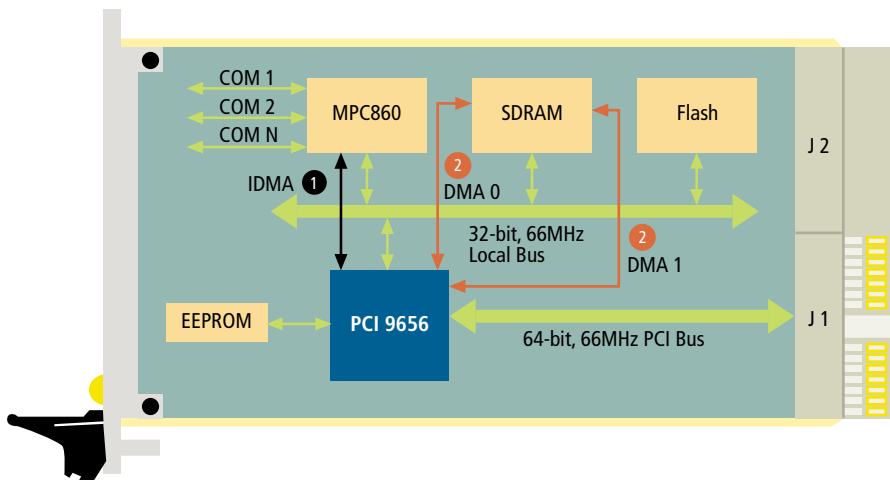
PCI 9656 PowerQUICC CompactPCI Adapter
