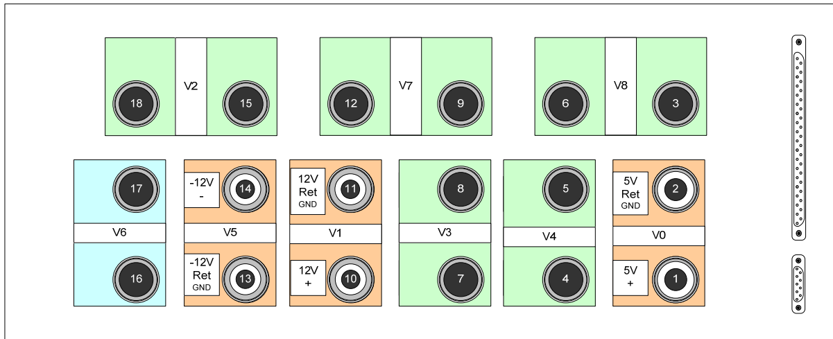
Fig. 4.4: Mod. V81XX VME64 configuration
