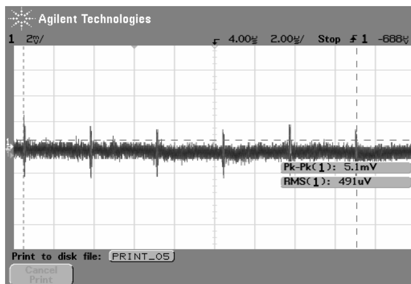
Fig. 4.9: Power Module ripple and noise measured at the output connector (@ 12V, 20A)
