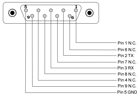
Fig. 5.3: RS-232 Connector (connector 9-pin DSUB female)
