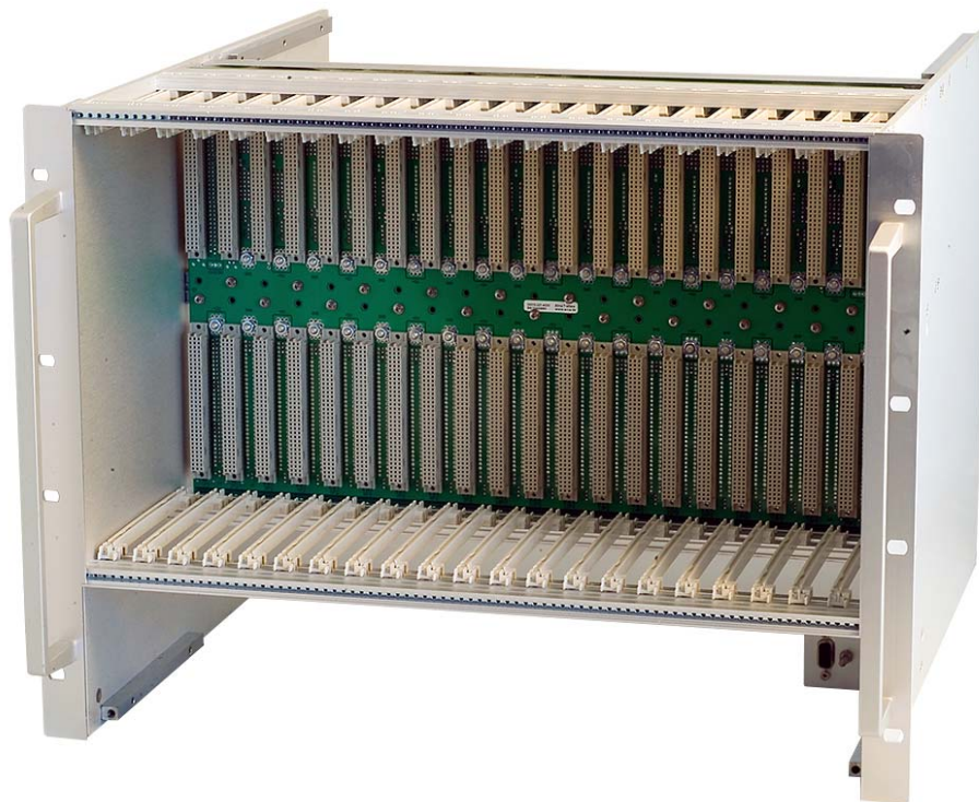
Fig. 3.1: Mod VME8100 Subrack (Bin + Backplane) front view
