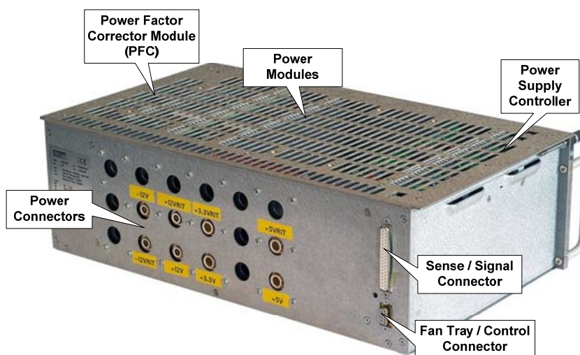
Fig. 4.2: Mod. V81XX Power Supplies components
