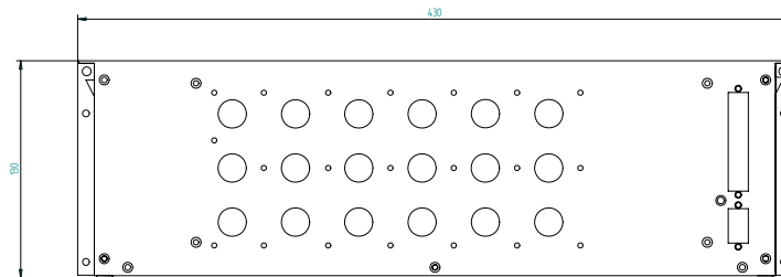
Fig. 2.4: Mod. V81XX Power Supply Front view
