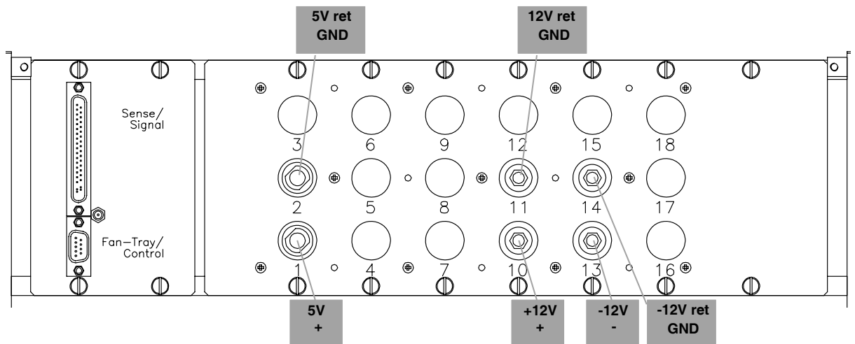
Fig. 3.4: Mod VME8100 Bin power connectors VME64
