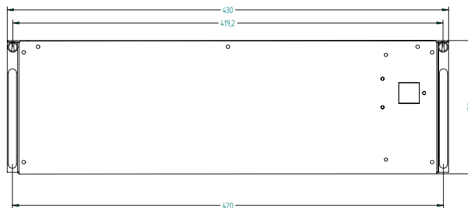
Fig. 2.5 Mod. V81XX Power Supply Rear view
