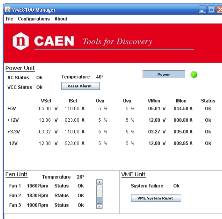
Fig. 7.5: Mod. VME8100_Manager Status/Set window (power ON)
