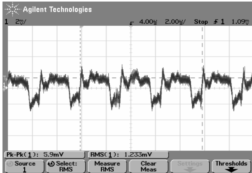
Fig. 4.7: Power Module ripple and noise measured at the output connector (@ 5V, 110A)
