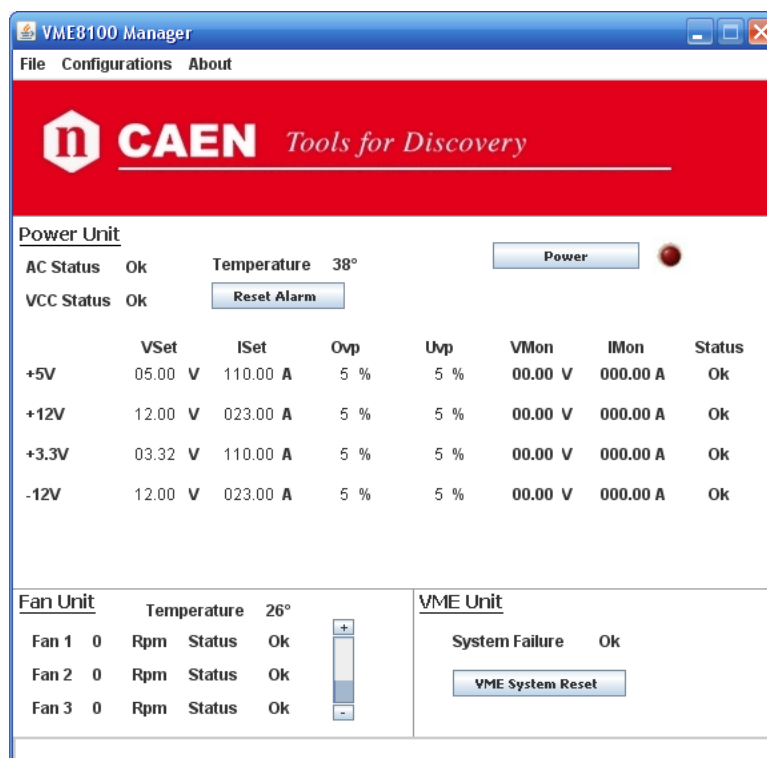
Fig. 7.4: Mod. VME8100_Manager Status/Set window (power off)
