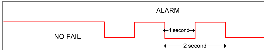
Fig. 5.6: FAIL signal timing
