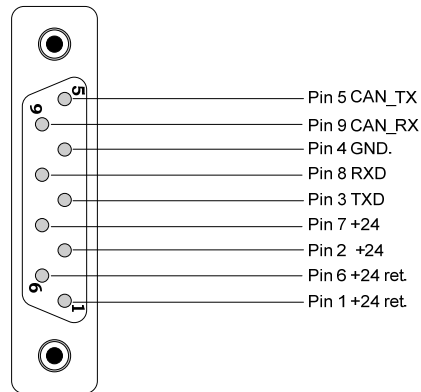
Fig. 4.11: Fan Tray / Control Connector ( 9-pin DSUB female)
